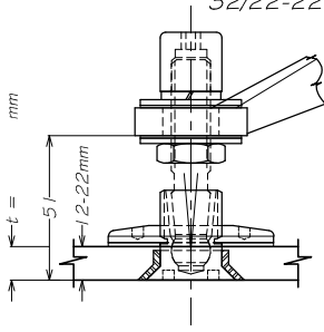
32/22-22n SWIVEL
